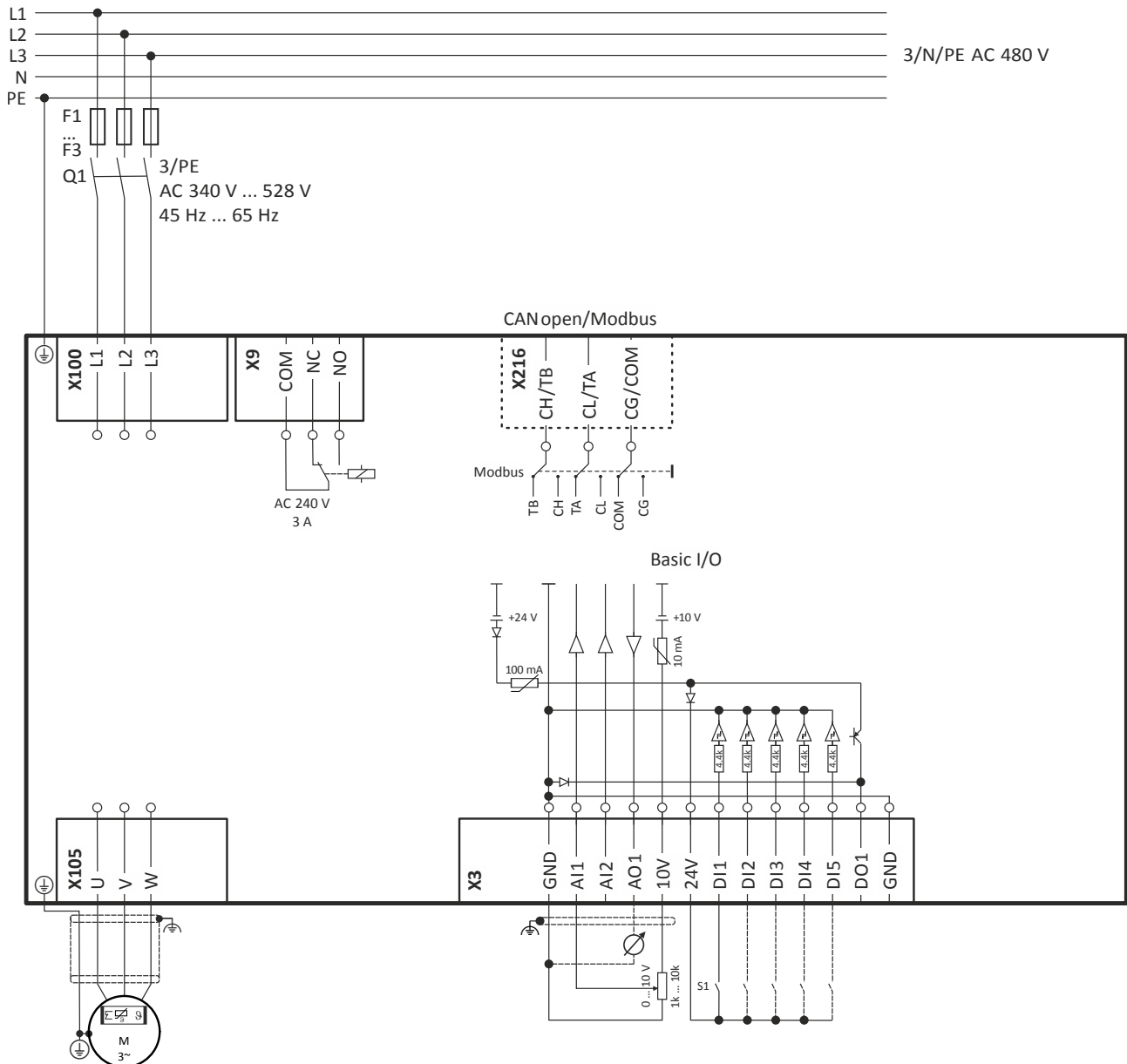
Fig. 6: Wiring example
