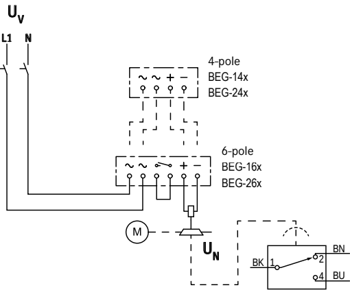
Supply: Phase-N
