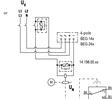
Supply: Phase-Phase or Phase-N by 4-pole rectifier
