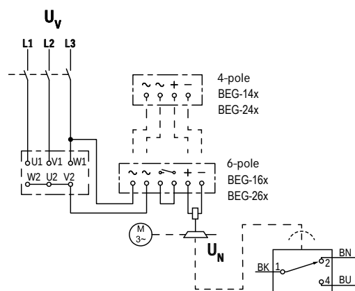
Supply: Phase-Starpoint
