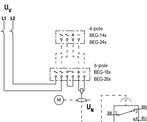
Supply: Phase-Phase
