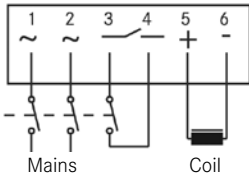
DC switching
