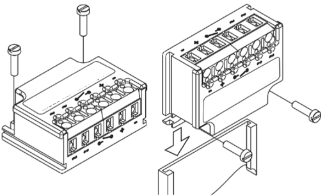
AC switching
